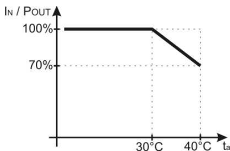
Graph 1. Relation between output current and ambient temperature.
