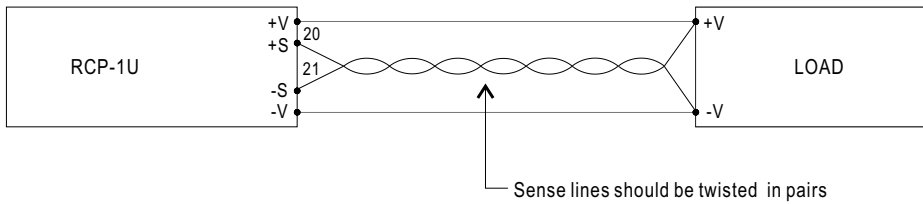
Sense lines should be twisted in pairs
